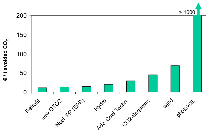
Costs of CO 2 -Emissions avoided by specific measures
