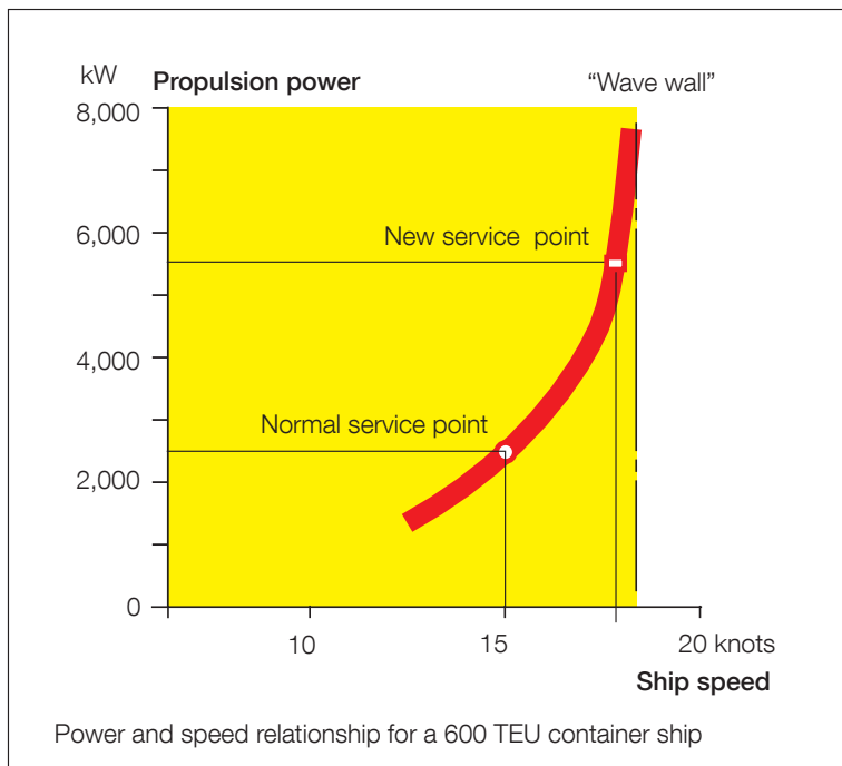
Fig. 5: The “wave wall” ship speed barrier
