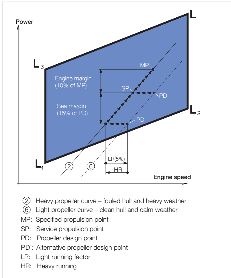
Fig. 17: Ship propulsion running points and engine layout
