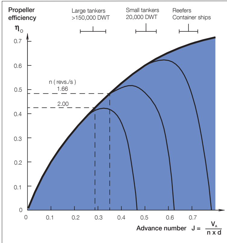
Fig. 8: Obtainable propeller efficiency – open water, Ref. [3], page 213
