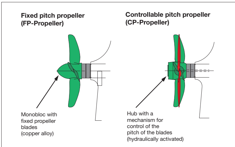
Fig. 7: Propeller types
