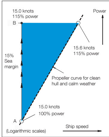
Fig. 12a: Ship speed performance at 15% sea margin
