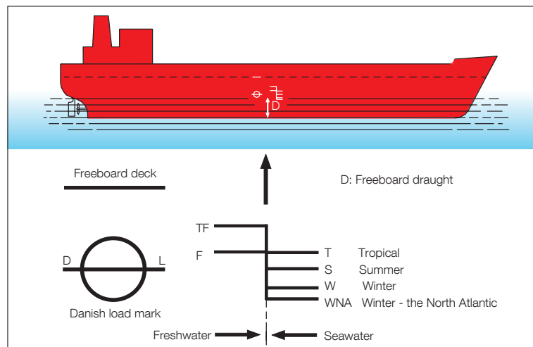
Fig. 1: Load lines – freeboard draught
