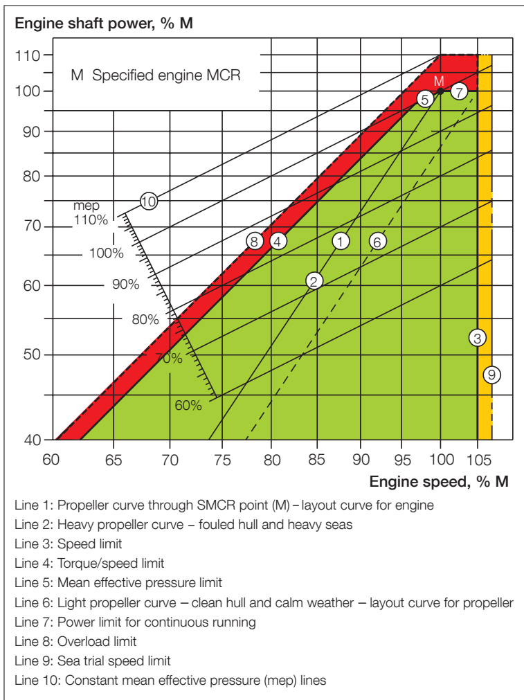
Fig. 18: Standard engine load diagram
