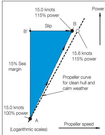
Fig. 12b: Propeller speed performance at 15% sea margin
