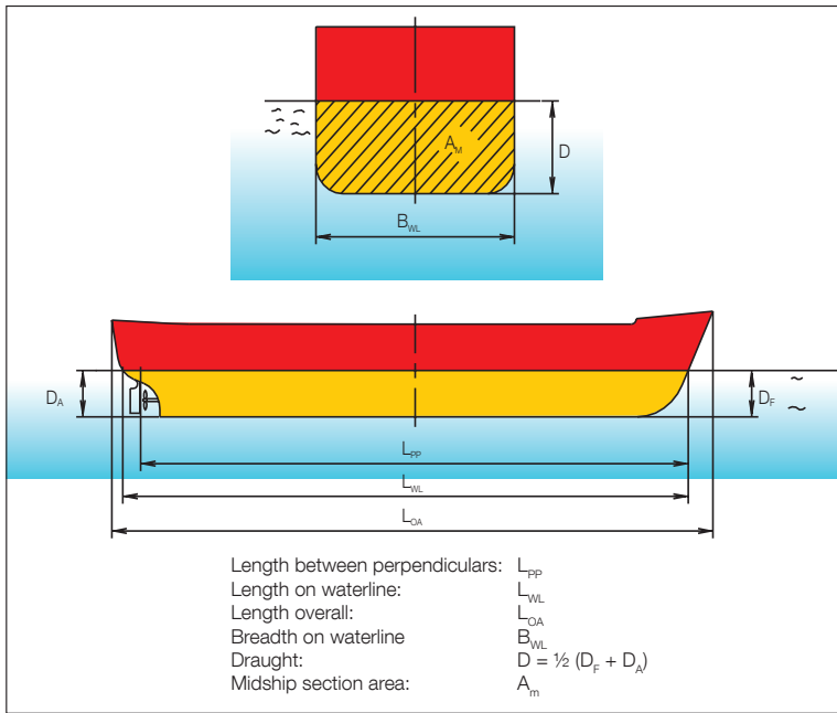
Fig. 2: Hull dimensions
