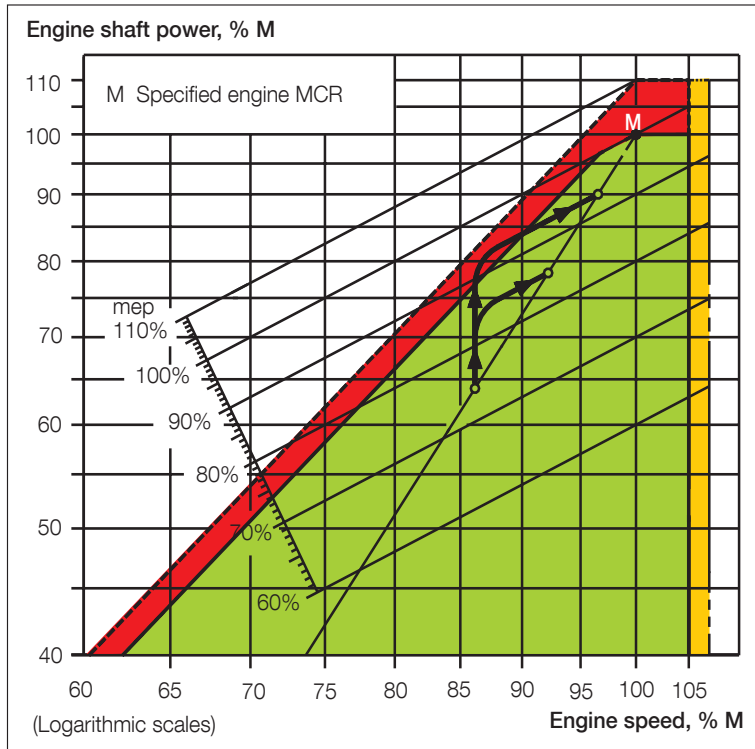
Fig. 15: Load diagram – acceleration
