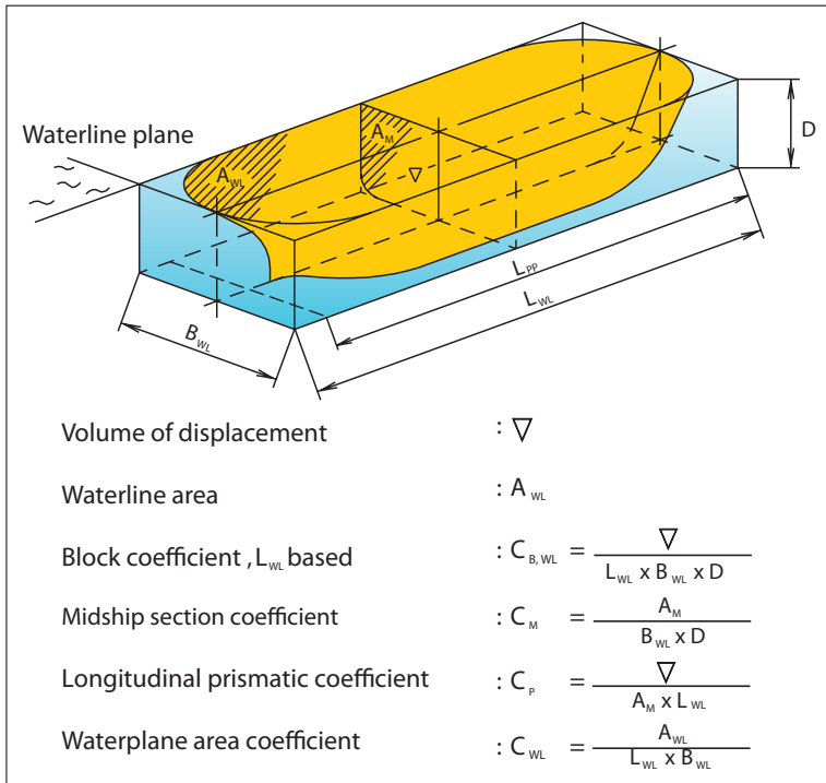
Fig. 3: Hull coefficients of a ship
