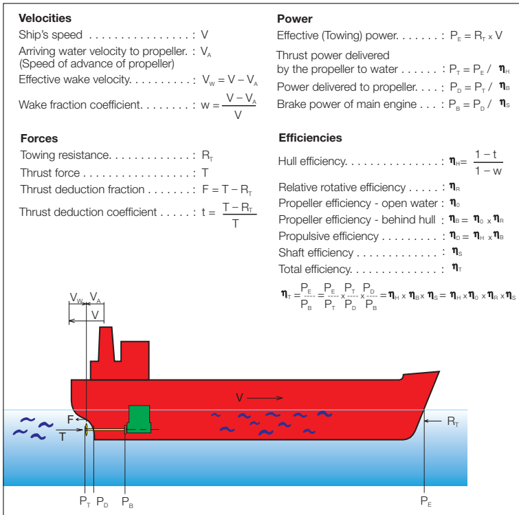
Fig. 6: The propulsion of a ship – theory
