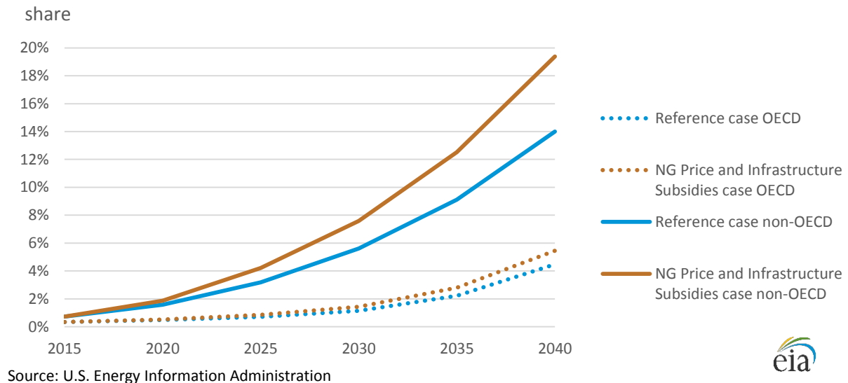
Figure 36. Updated ITEDD Reference case and Natural Gas Price and Infrastructure Subsidies case medium- and heavy-duty vehicle natural gas consumption shares in OECD and non-OECD regions
