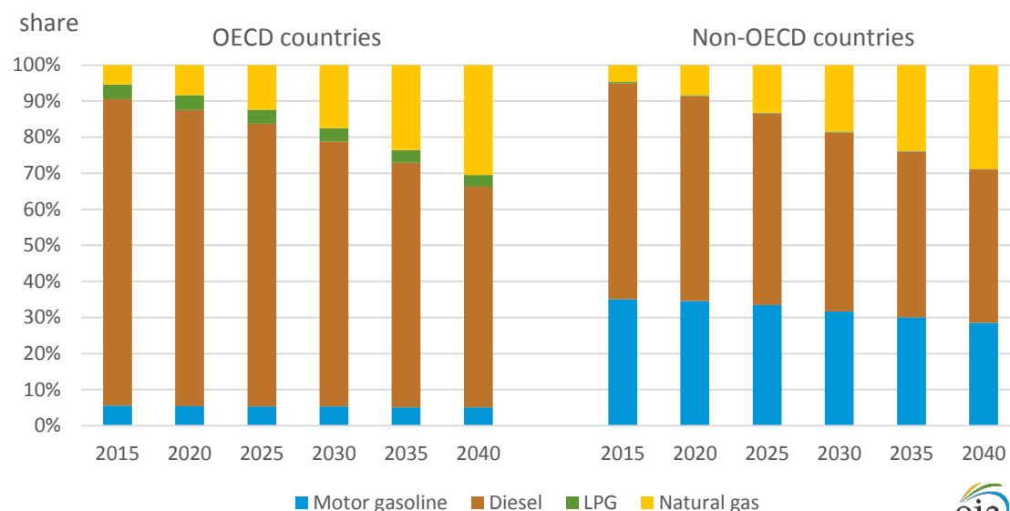
Figure 30. Updated ITEDD Reference case bus energy consumption shares in OECD and non-OECD countries
