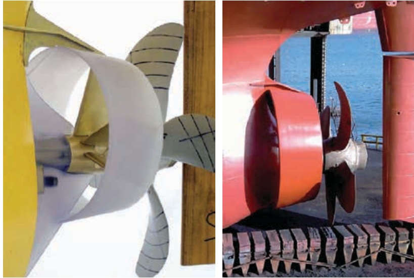
Figure 11. Becker Mewis Duct on a Bulk Carrier
