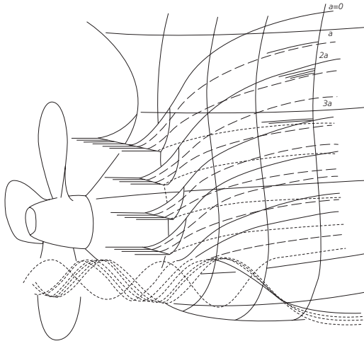
Figure 7. Grothues Spoilers Working Principle
