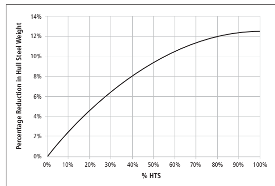
Figure 36. HTS Percentage of Weight Savings
