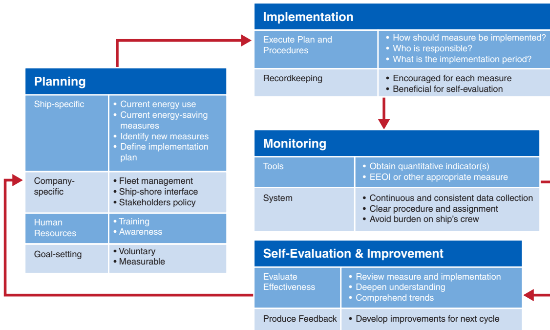
Figure 62. Four-step Continuous Improvement Process
