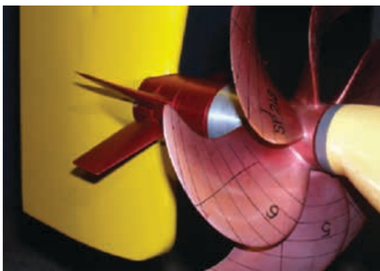
Figure 14. SHI Port-stator
