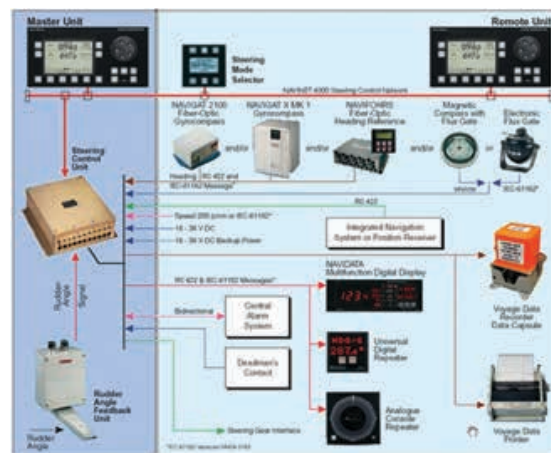
Figure 58. Self-tuning Adaptive Heading Control System (Sperry's NAVIPILOT 4000)
