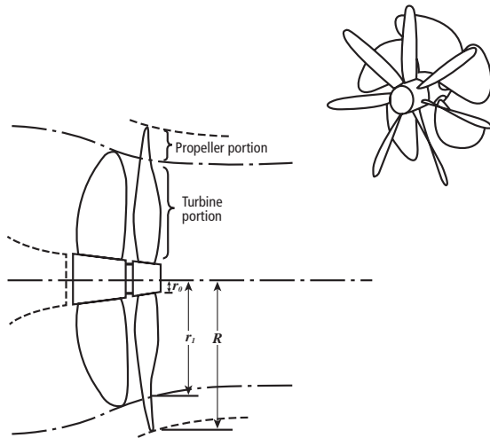
Figure 16. Grim Wheel Basic Principle
