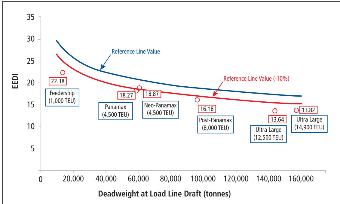
Figure 6. EEDI Assessment for Typical Containerships
