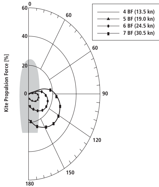
Figure 25. Relative Kite Propulsion Polar Plot
