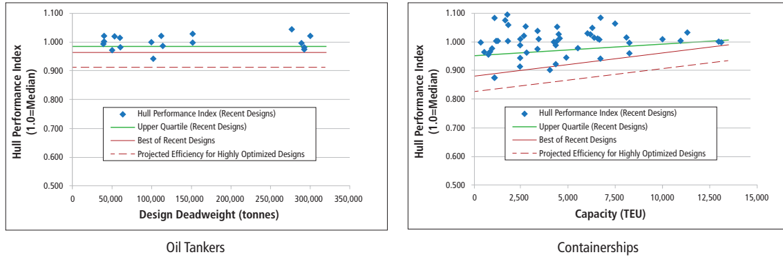
Figure 3. Hull Performance Comparison
