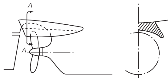
Figure 9. Partial-duct Stern Tunnel
