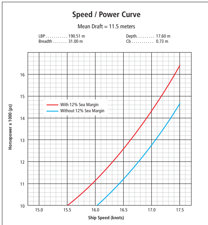
Figure 55. Typical Speed/power Curve
