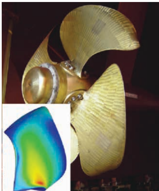
Figure 17. MAN Alpha Propellers with Kappel Blades
