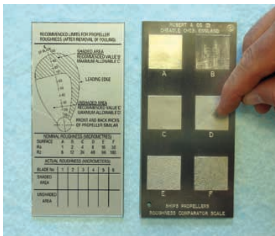
Figure 61. Rubert Propeller Roughness Comparator – Diver's Version
