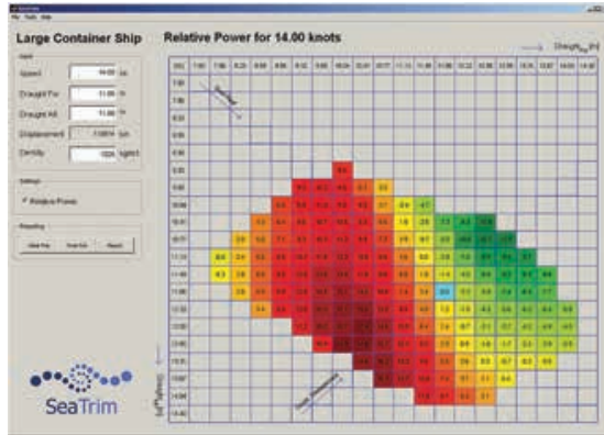
Figure 57. Sample Optimum Trim Calculator
