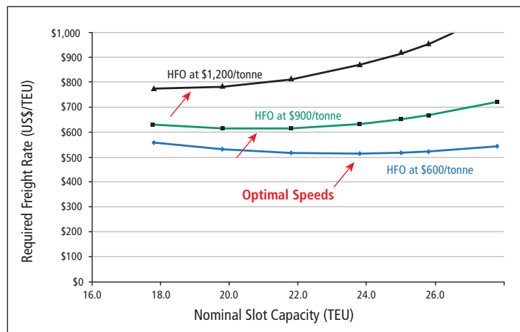
Figure 2. Containership Design Speed Parametric Study
