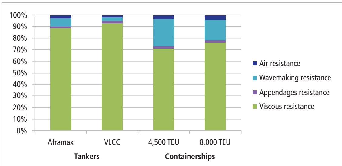
Figure 4. Components of Hull Resistance in Calm Water Conditions at Design Speed
