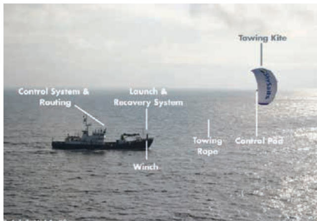
Figure 24. Towing Kite System on the MS BEAUFORT
