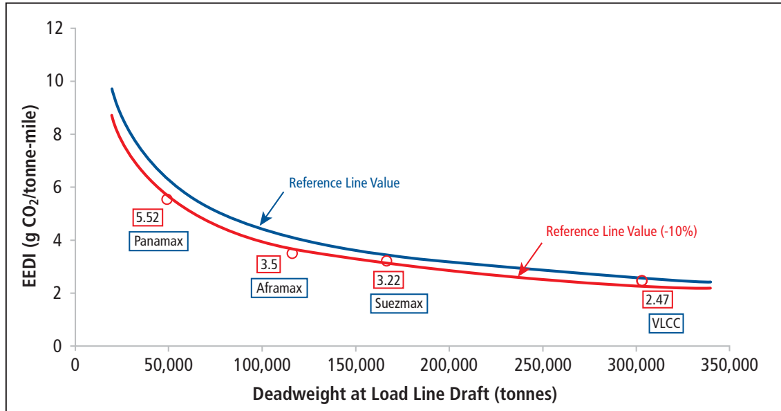
Figure 5. EEDI Assessment for Standard Tankers
