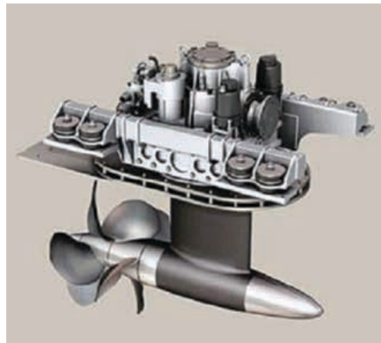
Figure 18. Contra-rotating Propellers on a Large Yacht Pod
