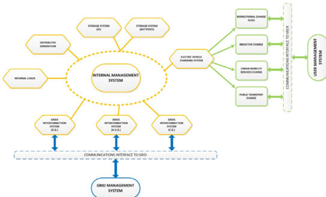
Figure 2. Full scale implementation of Smart Grids in Railway Infrastructure. Source: Win Inertia (2013).
