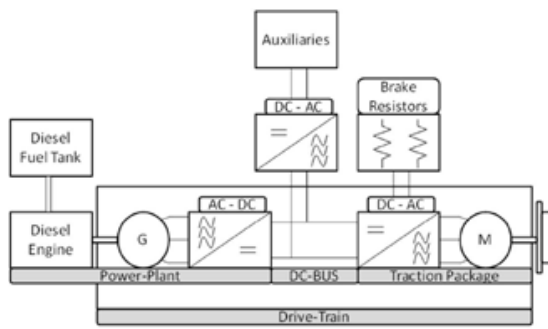
Figure 2. Diesel-electric drive system. Source: Hoffrichter, A (2013).
