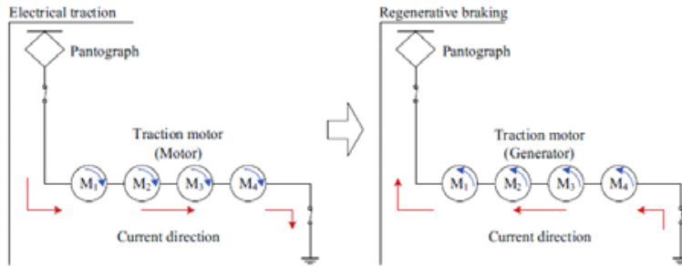
Figure 1. Principle of regenerative braking. Source: Xin Yang, et al (2015).
