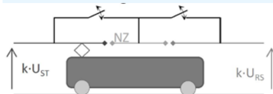
Figure 4. Bypass to be avoided that determines NZ length. Source: Pilo, E. (2014).
