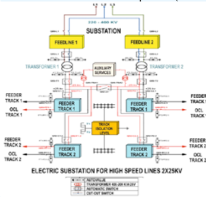
Figure 2. 2x25 scheme. Source: Adif. (2016).
