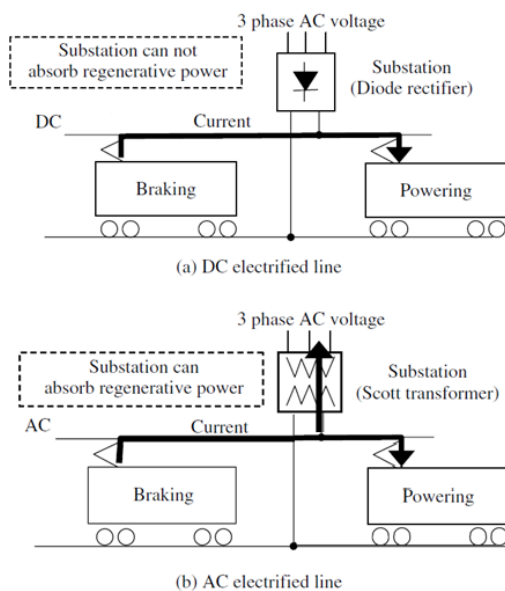
Figure 3. Regenerated energy flow in each electrified line. Source: Keiichiro Kondo (2010).
