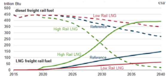
Figure 4. Comparison of energy consumption for freight rail using diesel and LNG (2015-40). Source: N. Chase(2014).
