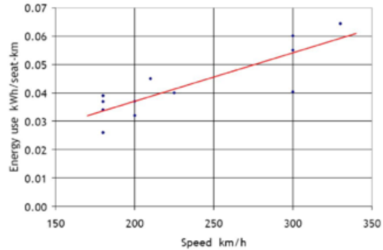
Figure 1: Relationship between energy consumption and speed in rail vehicles. Source: RSSB, T618 Traction Energy Metrics (2007).
