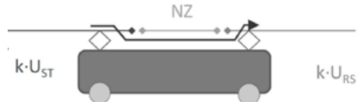
Figure 1. Bypass to be avoided that determines NZ length. Source: Pilo, E. (2014).
