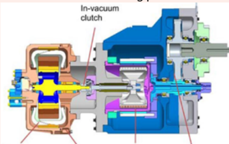
Figure 2. Section of flywheel assembly (for test ring). Source: Wheals, J. C. et al. (2015).
