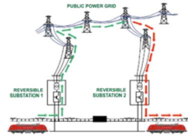
Figure 1. Energy flow in railways. Source: Adif. (2016).
