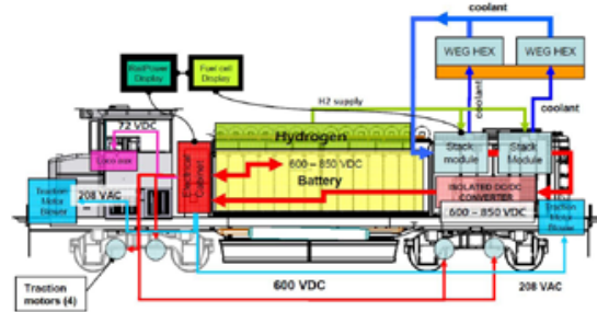
Figure 5. Hydrogen switcher's diagram. Source: Miller, A. R. (2007).
