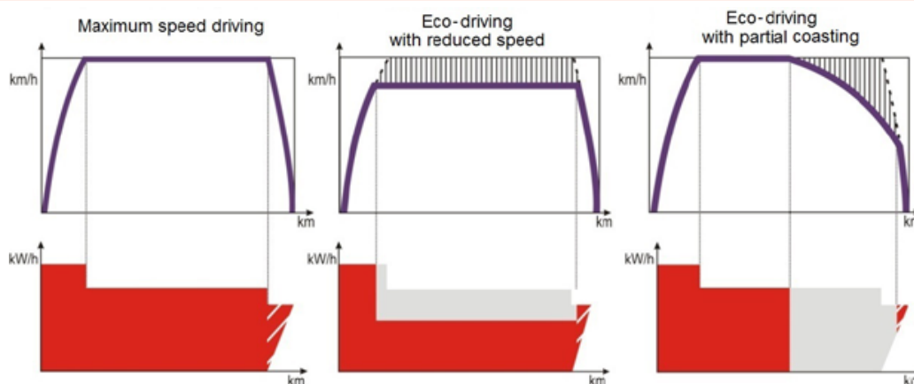
Figure 3a: Different driving strategies. Source: García, A. (2016).
