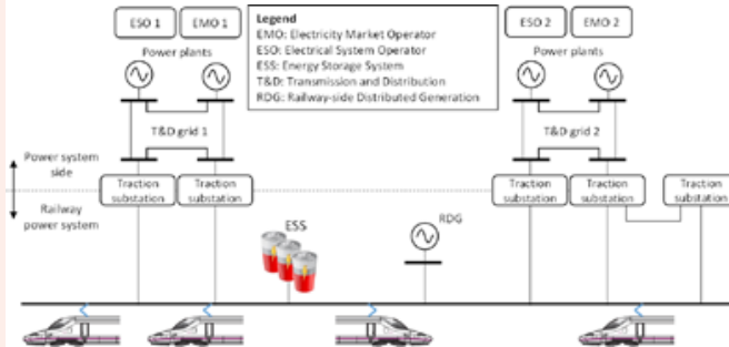
Figure 1. Physical description on interrelations among railways power systems and public grids. Source: MERLIN Project (2015). WP2. Study of the business models in scenario 3.
