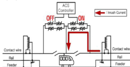
Figure 5. Electric railway system with ACS system and SFCL.. Source: Hee-Sang Shin (2011).
