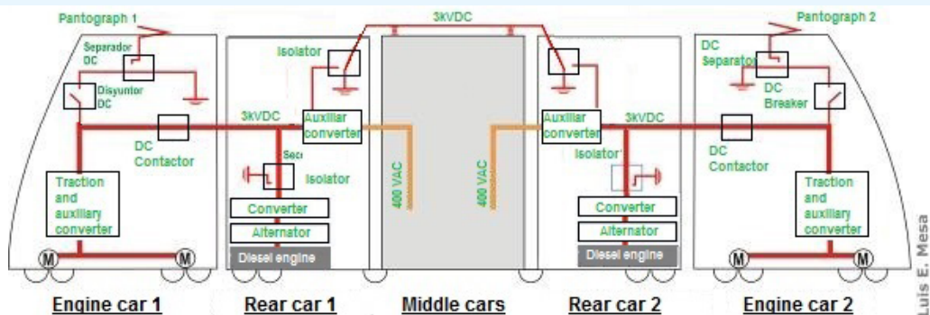
Figure 3. Dual passenger train supplied by diesel. Source: Gonzalez Franco, I et al. (2010).
