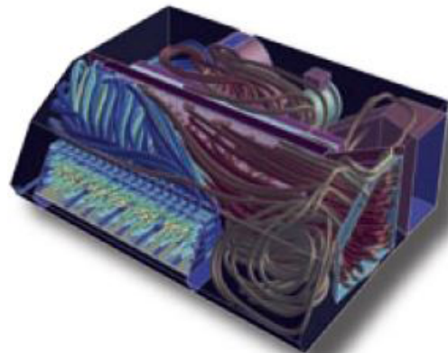
Figure 3. Computational Fluid Dynamic (CFD) studies of HVAC unit. Source: Merak.
