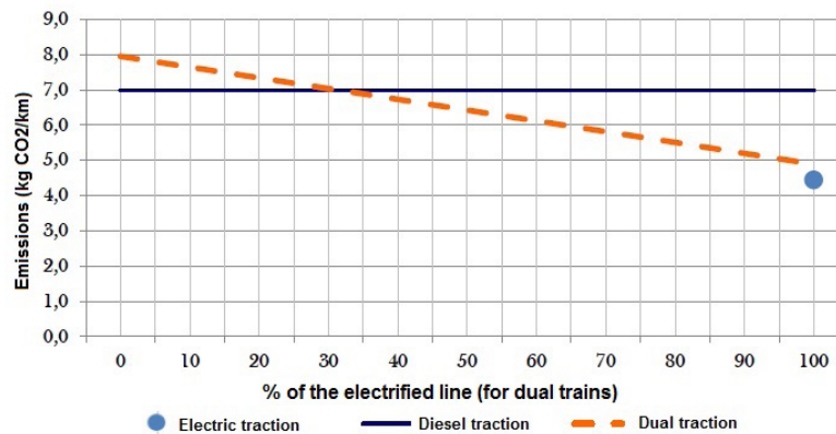
Figure 4. CO 2 emissions according to the electrified length in passenger transport. Source: Gonzalez Franco, I et al. (2010).
