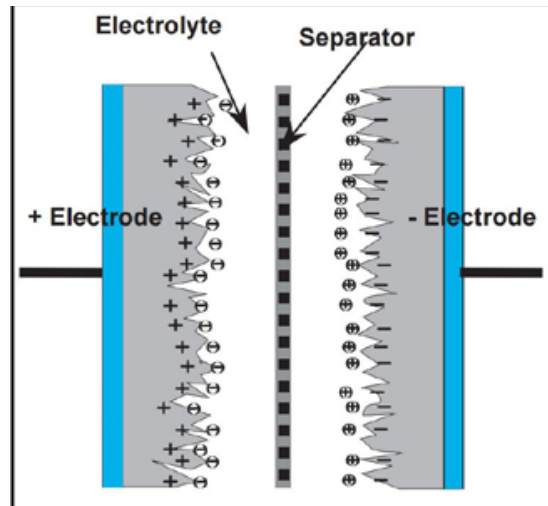
Figure 1. Ultracapacitor Charge Separation. Source: Maher, B et al. (2006).
