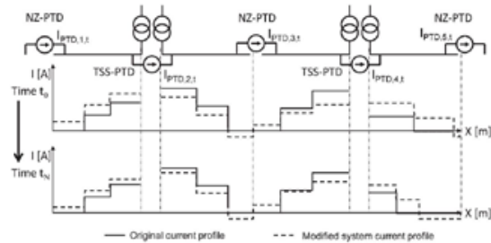
Figure 6. Per-phase current distribution along the catenary. Source: E.Pilo (2014).
