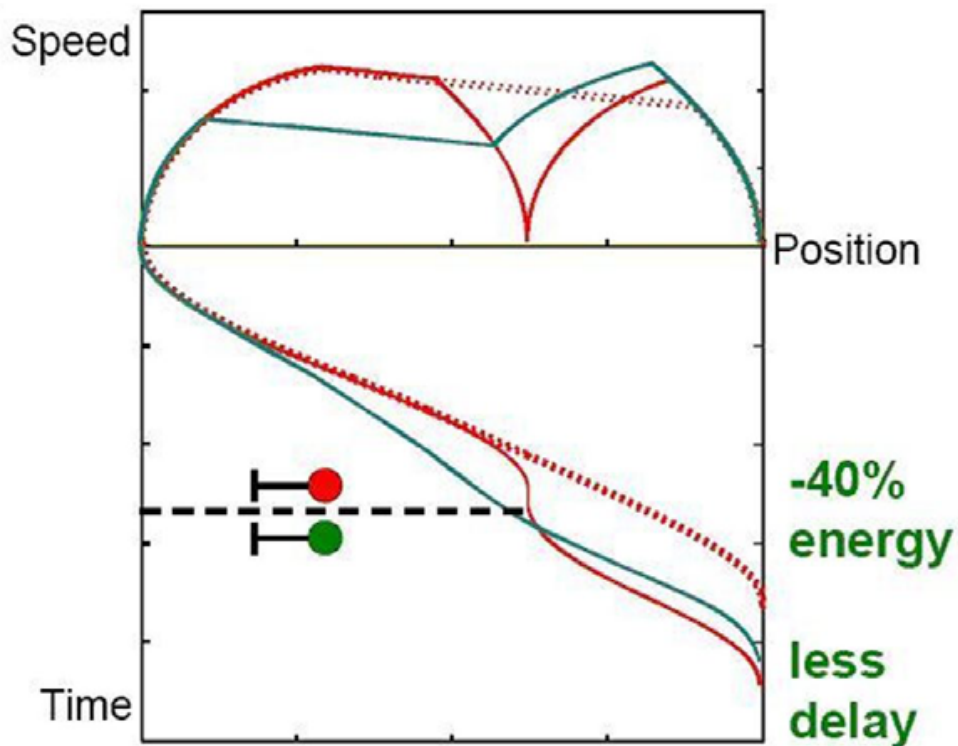
Figure 3. Speed profile of a non-optimal operation and an operation with a C-DAS. Source: Salvador, P. (2008).
