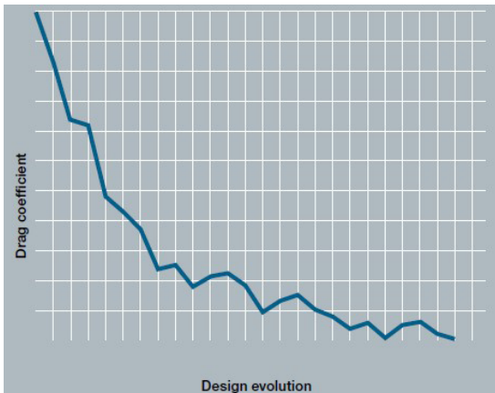
Figure 2: Iteration process from the initial design to the optimized shape. Source: Bombardier.
