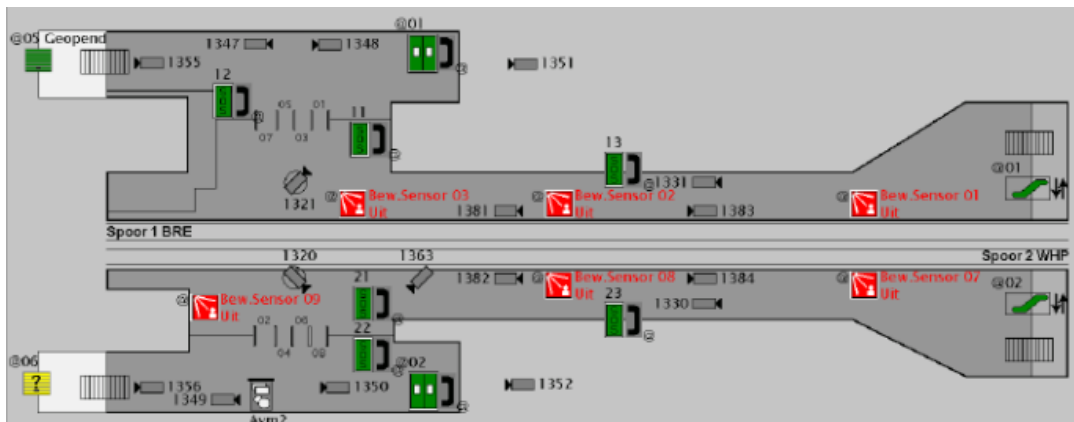
Figure 4: Layout of a smart lighting management using sensors in a railway station. Source: Ticket to Kyoto Project (2013).
