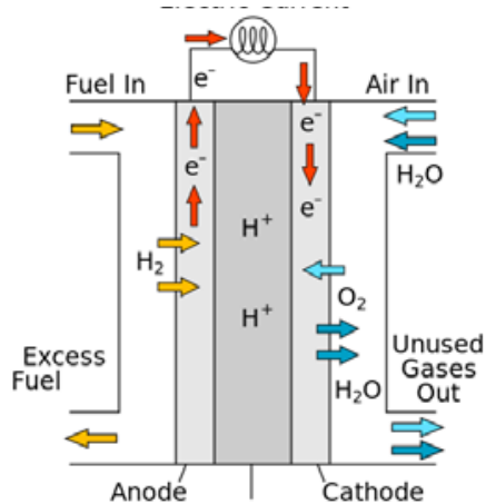
Figure 1. Fuel cell scheme. Source: Wikipedia (2012).
