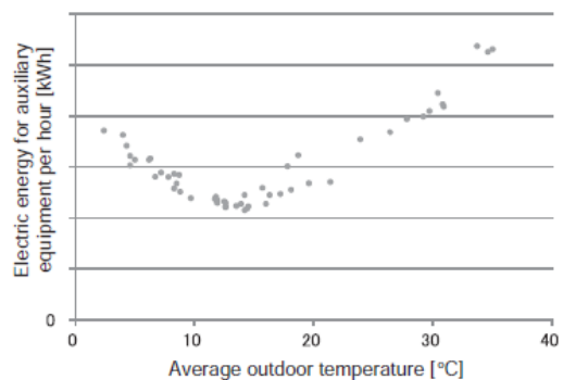
Figure 3: Outdoor temperature and electric energy of auxiliary equipment per hour. Source: Mizuguchi, Y. et al. (2015).
