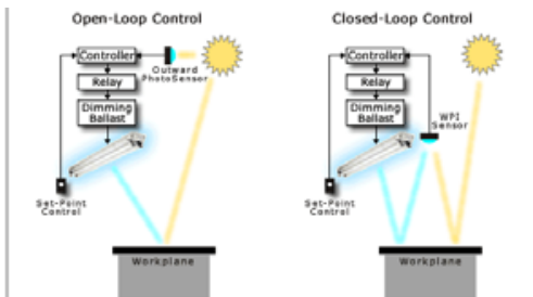
Figure 2: Categories of automatic daylight harvesting lighting controls. Source: IntelliBlinds.
