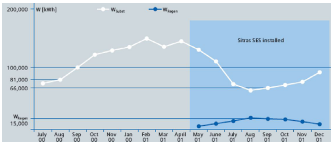
Figure 3: Energy consumption before and after the use of the SITRAS SES. Wilde, J. L. (2011).
