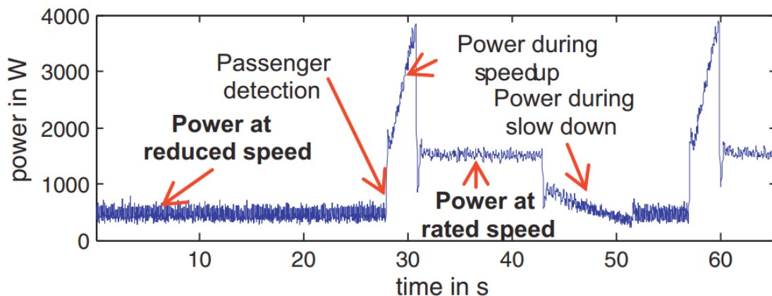
Figure 2: Power consumed by an escalator with two speed modes. Source: Carrillo et al. (2013).
