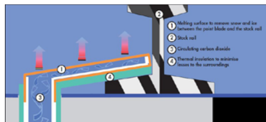
Figure 3: Scheme of a rail heated with geothermal energy. Source: BINE.
