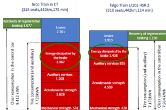
Figure 4: Comparison of the energy consumption disaggregated by a high speed train (right) and conventional train (left). Source: García Alvarez, A (2009).
