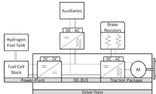
Figure 3. Hydrogen drive system. Source: Hoffrichter, A (2013).
