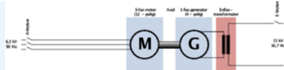
Figure 3. In-principle structure of a rotary frequency converter. Source: Merlín (2013).
