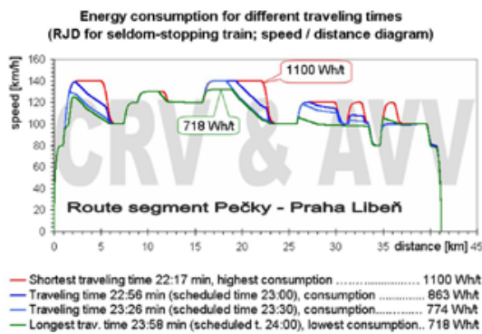
Figure 4: Energy consumption for different travel times I. Source: Salvador, P. (2008).
