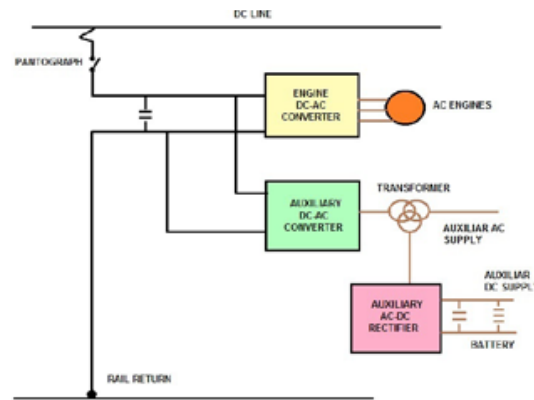
Figure 3. DC line power equipment. Source: own elaboration. (2016).
