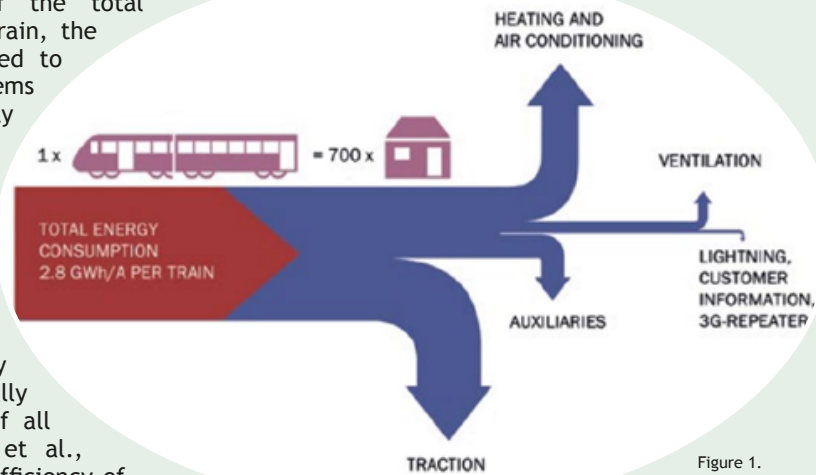
Figure 1. Example of energy consumption distribution on a train. Source: UIC Handbook 2015.
