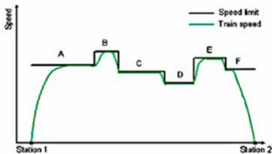
Figure 1. Shortest time driving strategy (hypothetical example). Source: Salvador, P. (2008).
