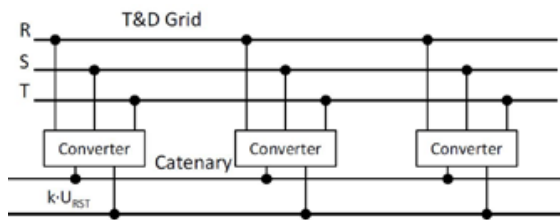
Figure 3. Power-supply system using converter . Source: Pilo, E. (2014).
