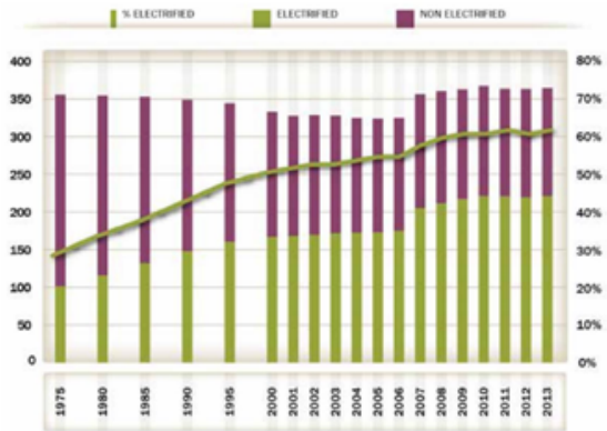
Figure 2. Length and share of electrified and non-electrified railway tracks, 1975-2013 (thousand km). Source: Railway Hand Book 2016.
