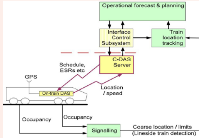
Figure 1. C-DAS scheme Source Gershuny, E (2014)
