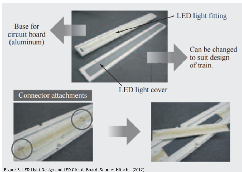
Figure 3. LED Light Design and LED Circuit Board. Source: Hitachi. (2012).
