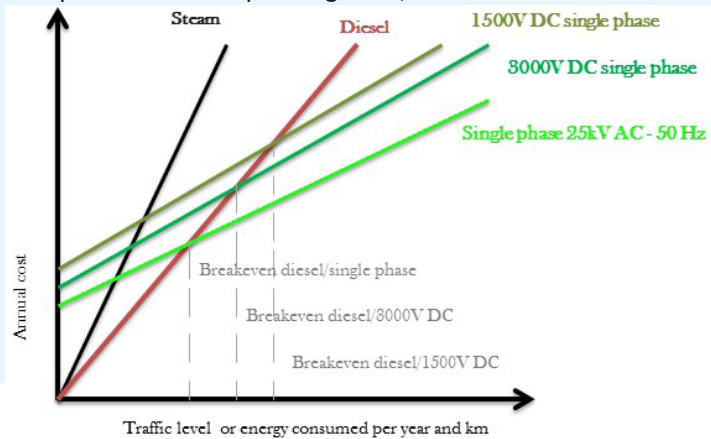
Figure 4. Costs comparison in different tractions. Source: Lopez Pita, A. (2008).
