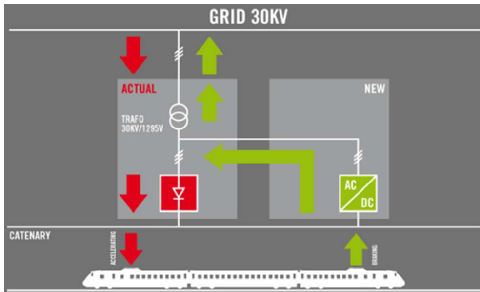
Figure 7. Reversible substation scheme. Source: Romo, A (2015).
