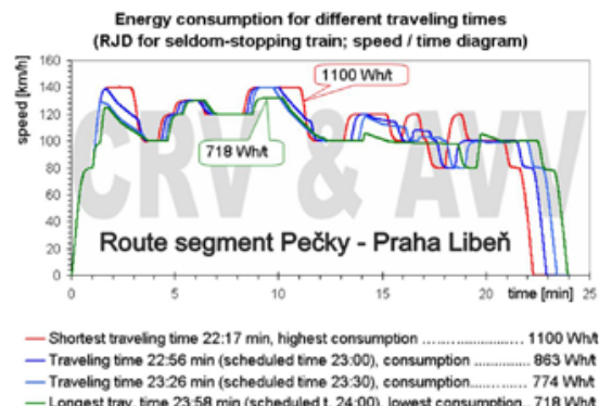
Figure 5: Energy consumption for different travel times II. Source: Salvador, P. (2008).
