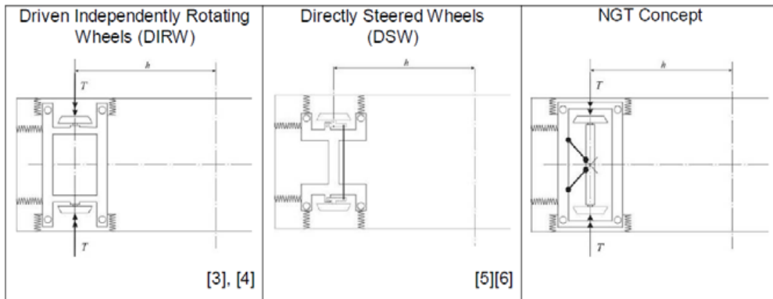
Figure 3: Steering principles for independently rotating wheels. Source: Robotics and Mechatronics Centre.
