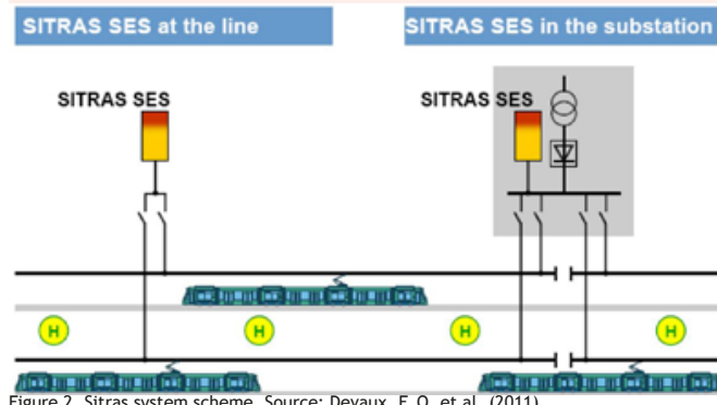
Figure 2. Sitras system scheme. Source: Devaux, F. O. et al. (2011).
