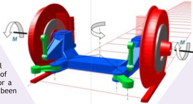
Figure 2: Unit with carrier and independently torque-controlled wheels for the mechatronic running gear. Source: Robotics and Mechatronics Center.
