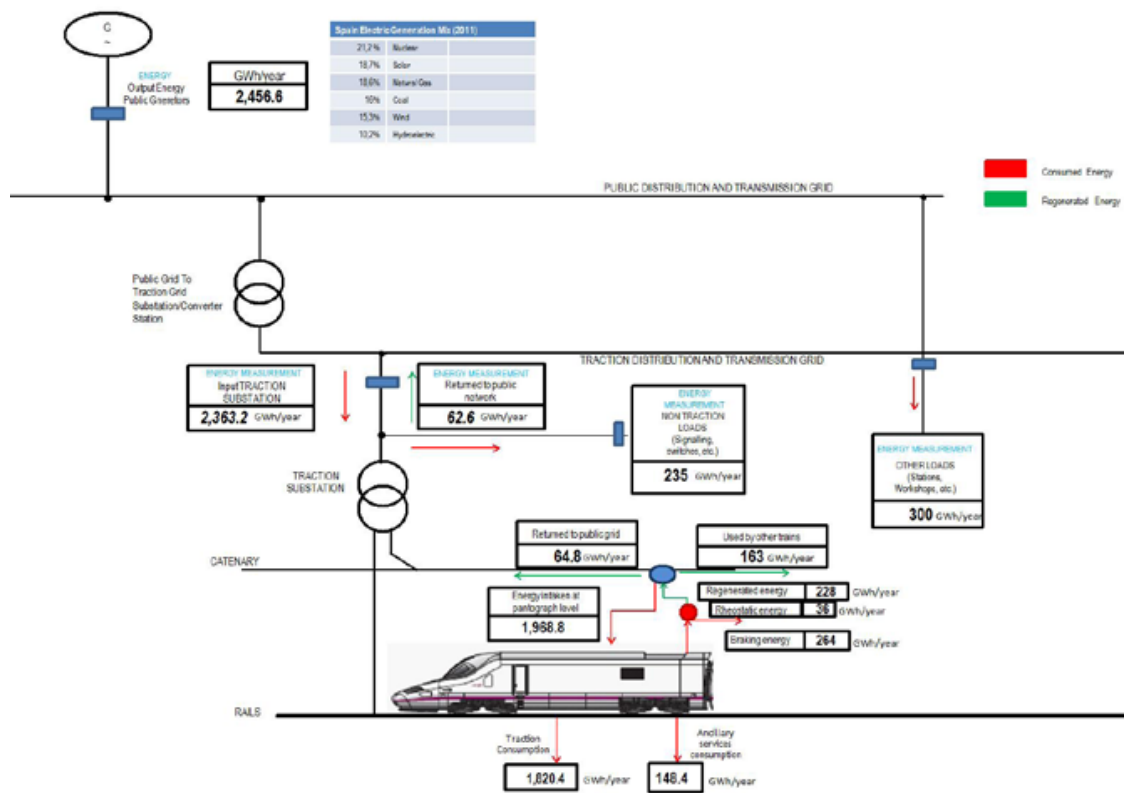
Figure 8. Energy flows for the Spanish case in 2011. Source: Merlin project.
