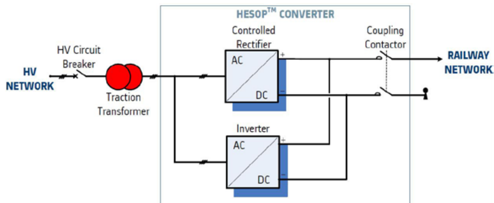
Figure 8. Architecture of the prototype power converter. Source: Cornic, D. (2010).
