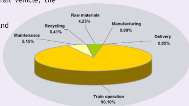
Figure 3: Energy consumption of a rail vehicle for the overall life cycle and 30 years of operation. Source: Siemens Transportation Systems (2006).
