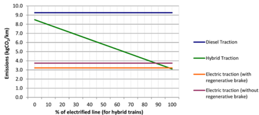
Figure 5. CO 2 emissions according to the electrified length in freight transport. Source: Gonzalez Franco, I et al. (2010).
