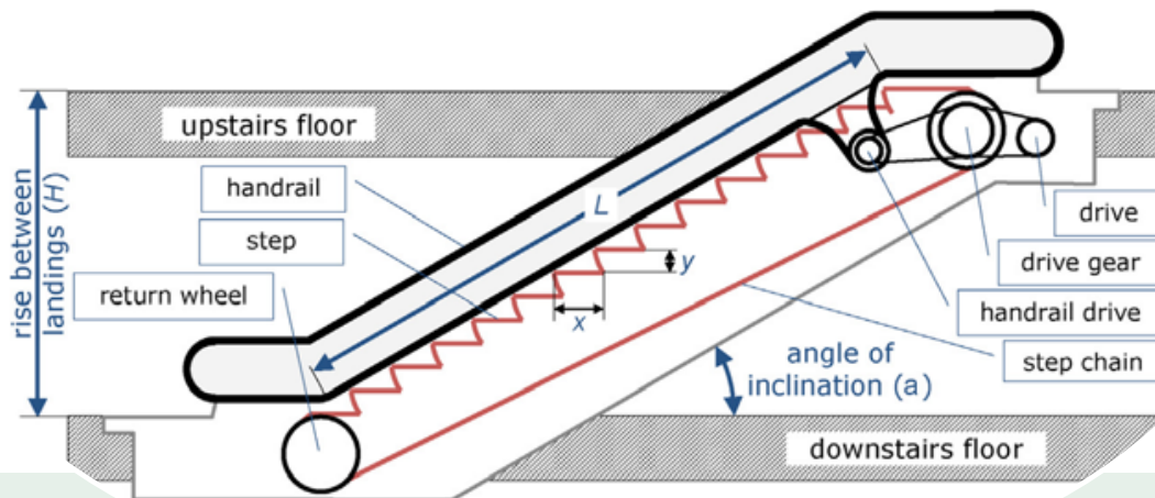
Figure 1: Escalator scheme. Source: Carrillo et al. (2013).
