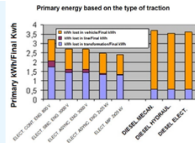
Figure 6. Comparison of primary energy for 1KWh of final energy. Source: García, A. (2016).
