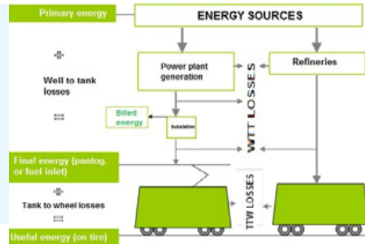
Figure 1. Primary, final and useful energy in operation. Source: García, A. (2016).
