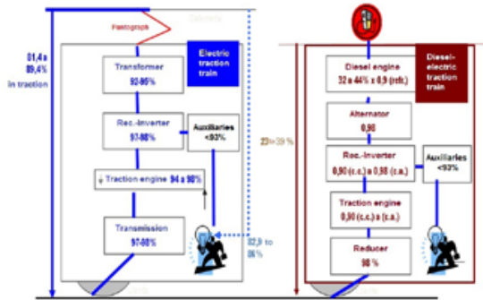
Figure 1. Tractor vehicles efficiency Source: García, A. (2016).
