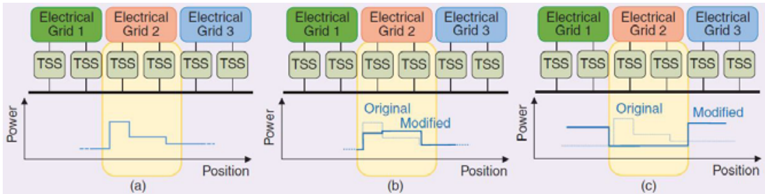
Figure 3. The different driving changes executed to manage the power demand in an RPS: (a) base case, (b) power peak reduction, and (c) energy transfer. Source: Pilo, E. et al. (2014).
