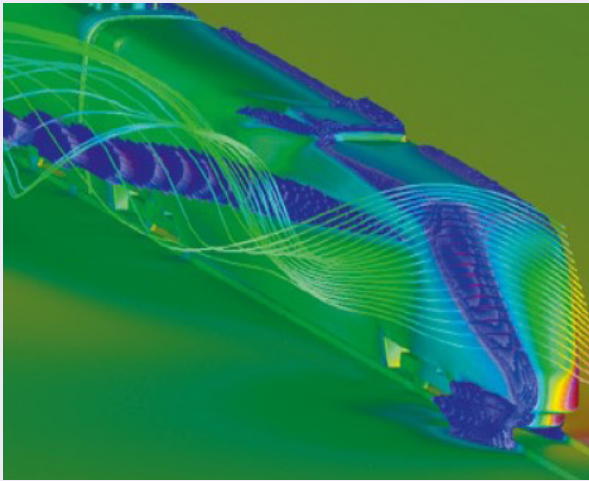
Figure 5: Visualization of flow ribbons - simulation of a high speed train running under cross-wind conditions. Source: Bombardier.
