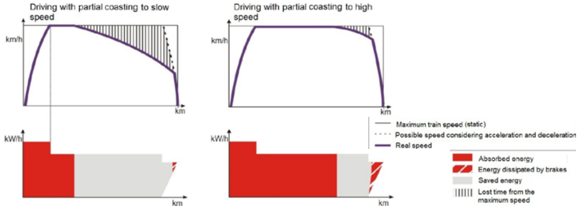
Figure 3b: Different driving strategies. Source: Garcia, A. (2016).
