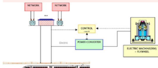
Figure 3. Schematic of the kinetic energy storage system and its implementation in a real track. Source: Iglesias, I. J.
