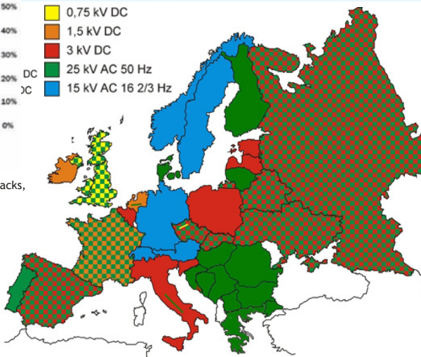
Figure 3. Types of electrification in Europe. Source: kolejpedia.
