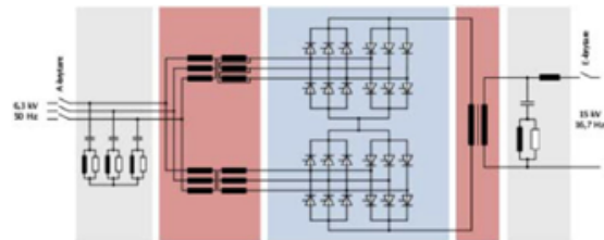
Figure 4. In-principle structure of a Cycloconverter. Source: Merlín (2013).
