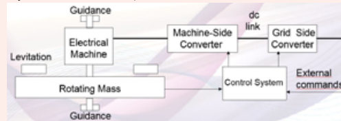
Figure 1. Flywheel scheme. Source: Lafoz, M. (2015).
