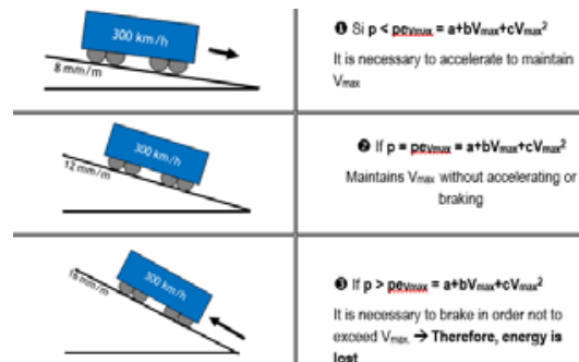
Figure 2a, 2b, 2c. Three possible cases for maintaining the maximum speed (300 km/h) on a downgrade. Source: González Franco, I. (2012).
