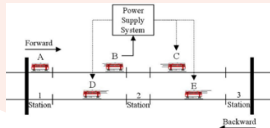
Figure 1. Group of stations. Source: K.M. Kim et al. (2010).
