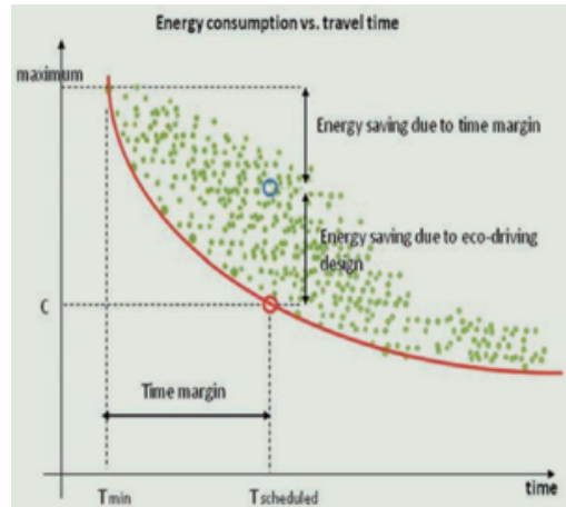
Figure 2. Relationship between travel time and energy consumption. Source: Cucala García, P et al. (2013).
