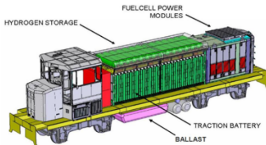
Figure 4. Hydrogen fuel cell CAD model Source: Miller, A. R. (2007).
