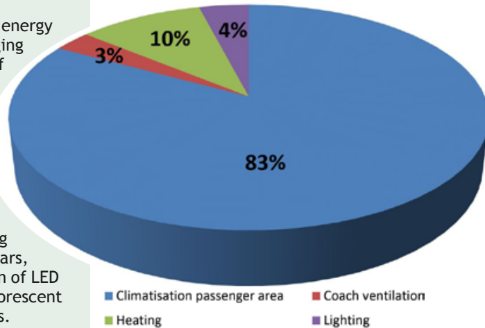
Figure 1. Energy demand of comfort functions in trains. Source: Knau (1993).
