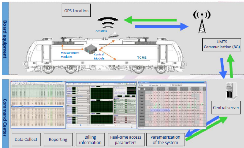
Figure 2: Scheme of the behaviour of the Bombardier metering device system. Source Vila, E. (2015).
