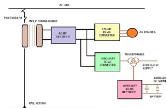
Figure 2. DC line power equipment. Source: own elaboration. (2016).
