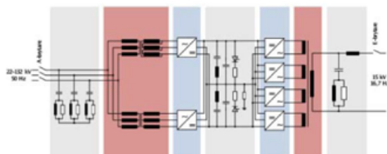
Figure 5. In-principle structure of DC-Link Converter Source: Merlín (2013).
