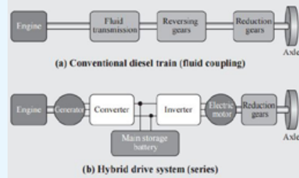
Figure 1: Traction System for Non-electrified Railway Lines. Diesel and hybrid trains components. Source: Shimada, M. et al. (2012).
