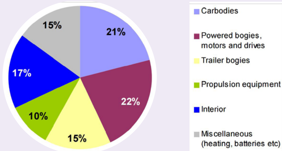
Figure 3: Typical breakdown of components in electric multiple unit trains by weight. Source: UIC EVENT (2003).
