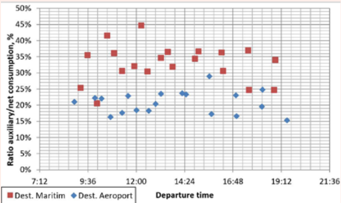
Figure 2: Ratio between auxiliary and net energy consumption in two lines of the Valencia Metro Network. Source: Martinez et al. (2015).
