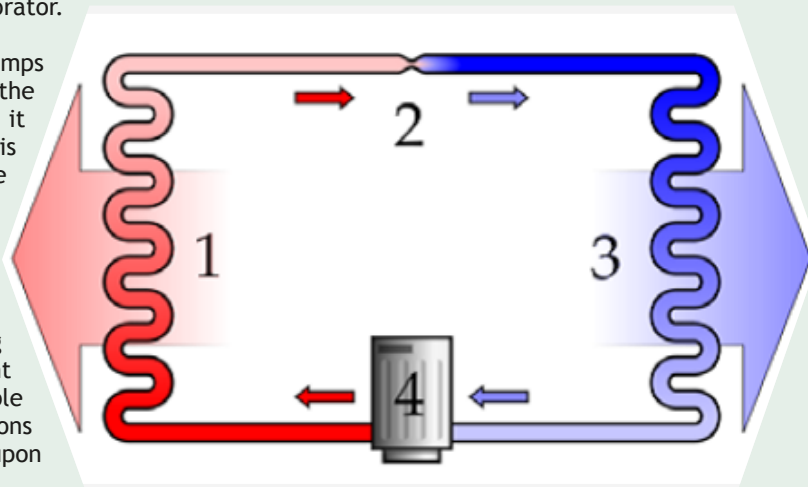
Figure 2. Basic HVAC configuration. 1) Condenser. 2) Expansion valve. 3) Evaporator. 4) Compressor. Source: Schaffler.
