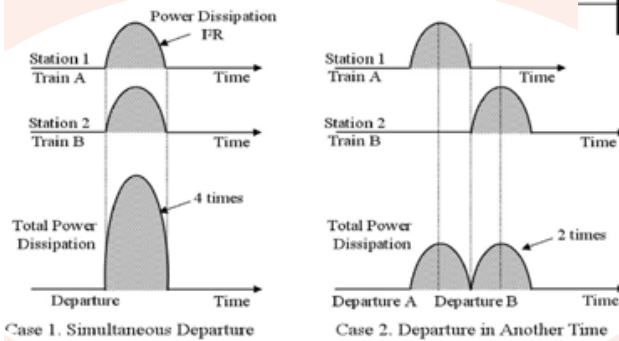
Figure 2. Power dissipation in traction phase. Source: K.M. Kim et al. (2010).
