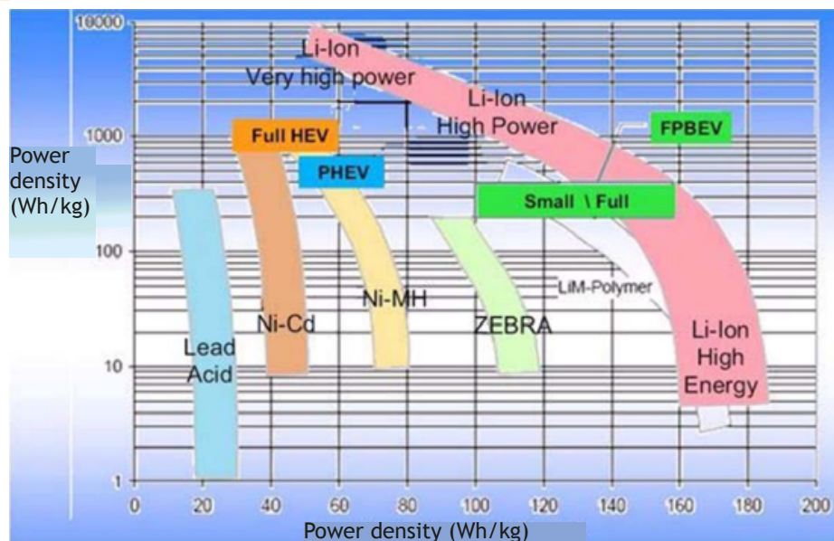
Figure 4: Relative power/energy density for different types of battery. Source: Estévez, P. et al. (2008).
