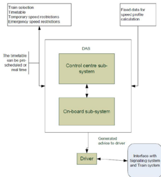
Figure 1. DAS architecture DAS. Source Jianhong Jin et al. (2011).
