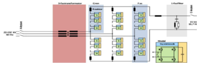
Figure 6. In-principle structures of Multi Level DC-Link converters. Source: Merlin (2013).
