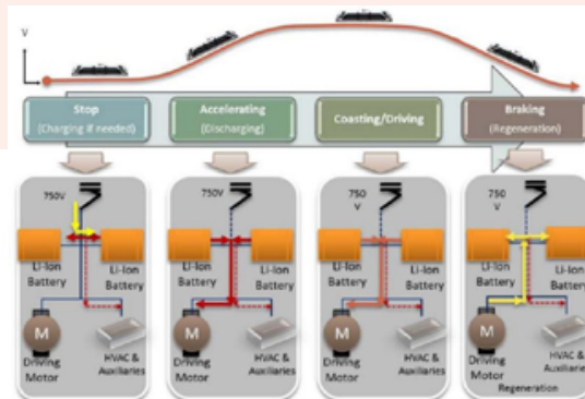
Figure 1 Operational steps of onboard battery-powered LRV
