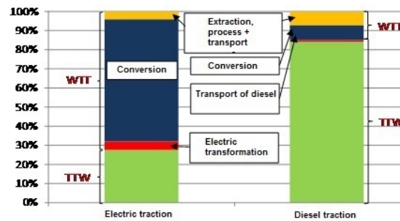
Figure 2. Percentage of energy by phases. Source: García, A. (2016).
