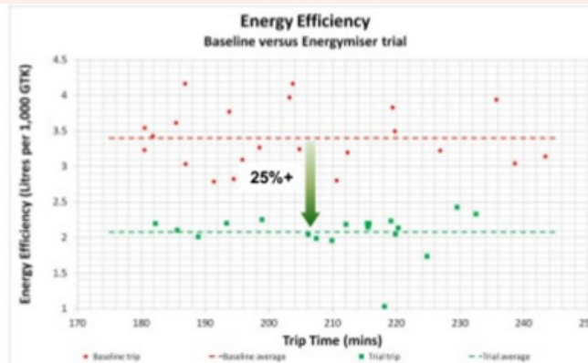
Figure 2. Results for 1500 T freight train. Source Guys, S. (2015).
