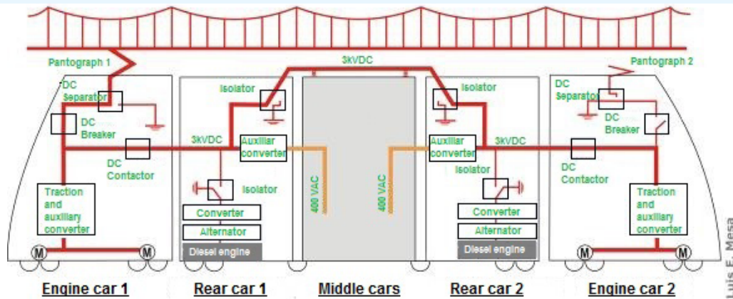
Figure 2. Dual passenger train supplied by electricity. Source: Gonzalez Franco, I et al. (2010).
