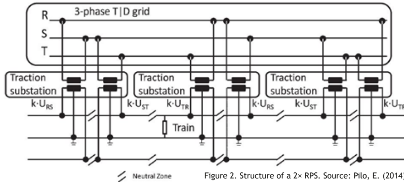
Figure 2. Structure of a 2x RPS. Source: Pilo, E. (2014).
