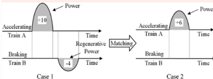
Figure 3. An example for synchronized driving. Source: K.M. Kim et al. (2010).
