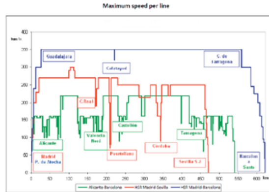
Figure 1. Maximum speed profile per route in several Spanish rail lines. Source: García, A. (2009).
