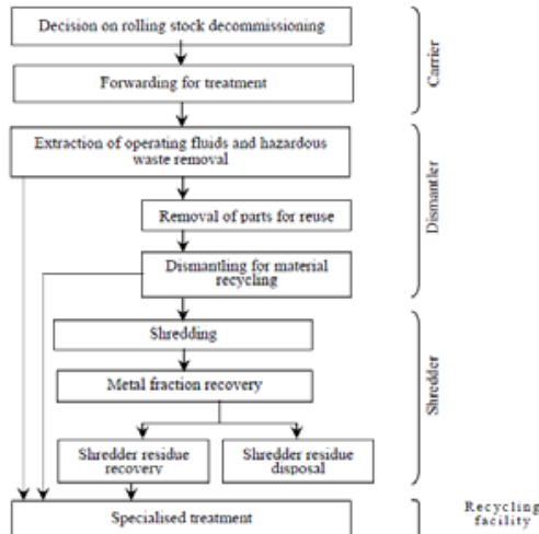
Figure 1. Recycling procedure for end-of-life rail vehicles. Source: WIT Transactions on The Built Environment (2014).
