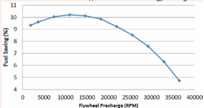
Figure 4: Effect of fly-wheel pre-charge on fuel savings. Source: Wheals, J. C. et al. (2015).
