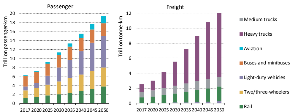
Figure 4.8 Passenger and freight transport activity by mode in India in the Base Scenario, 2017-50
