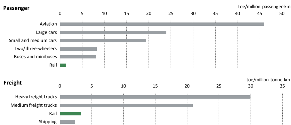
Figure 4.4 Energy intensity by transportation mode in India, 2017
