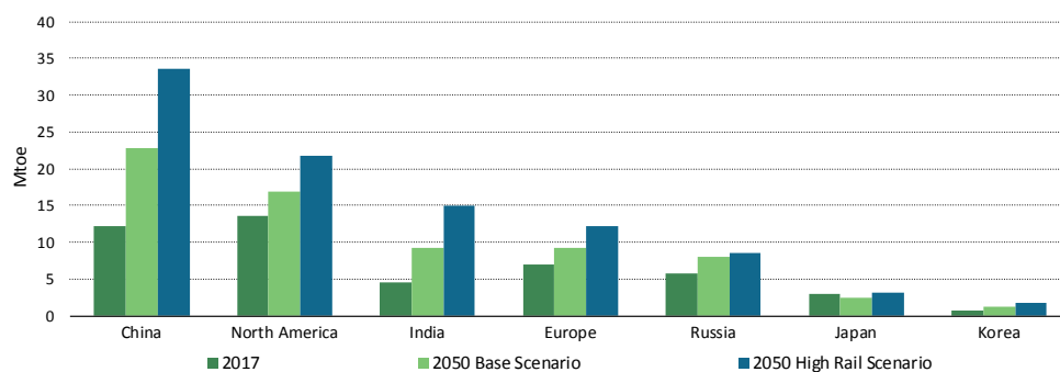
Figure 3.15 Projected rail energy demand growth by region
