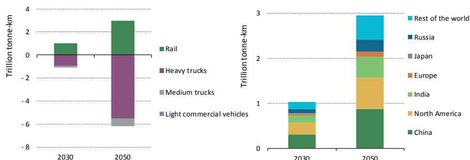
Figure 3.12 Change in surface freight transport activity (left) and freight rail activity (right) in the High Rail and Base scenarios, 2030 and 2050
