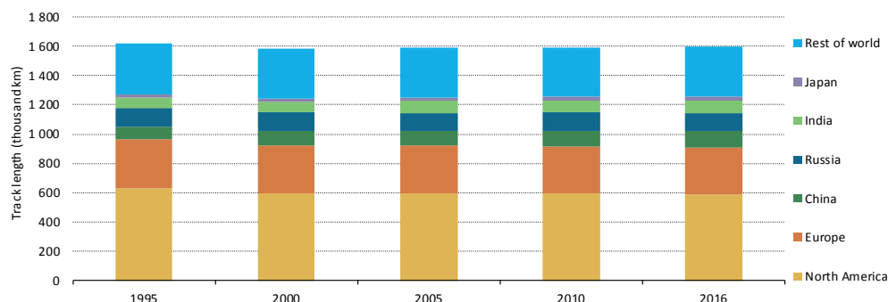
Figure 1.5 Conventional rail infrastructure track development, 1995-2016
