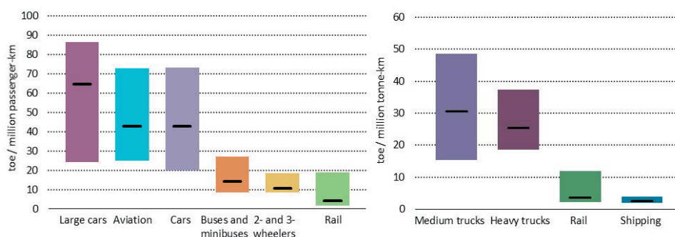
Figure 1.21 Energy intensity of different transport modes, 2017
