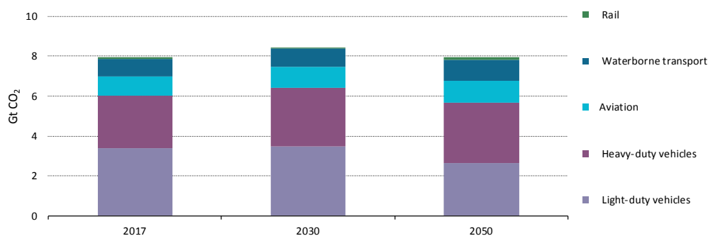
Figure 3.16 Direct CO 2 emissions from fuel combustion in the High Rail Scenario, 2017-50
