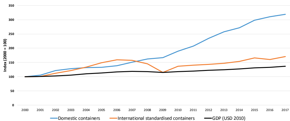
Figure 3.26 Number of containers used in intermodal transport relative to GDP in the United States, 2000-17
