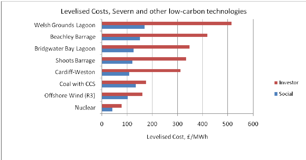
Figure 7: Levelised Energy Costs for Severn tidal power and other technologies, optimism bias included.
