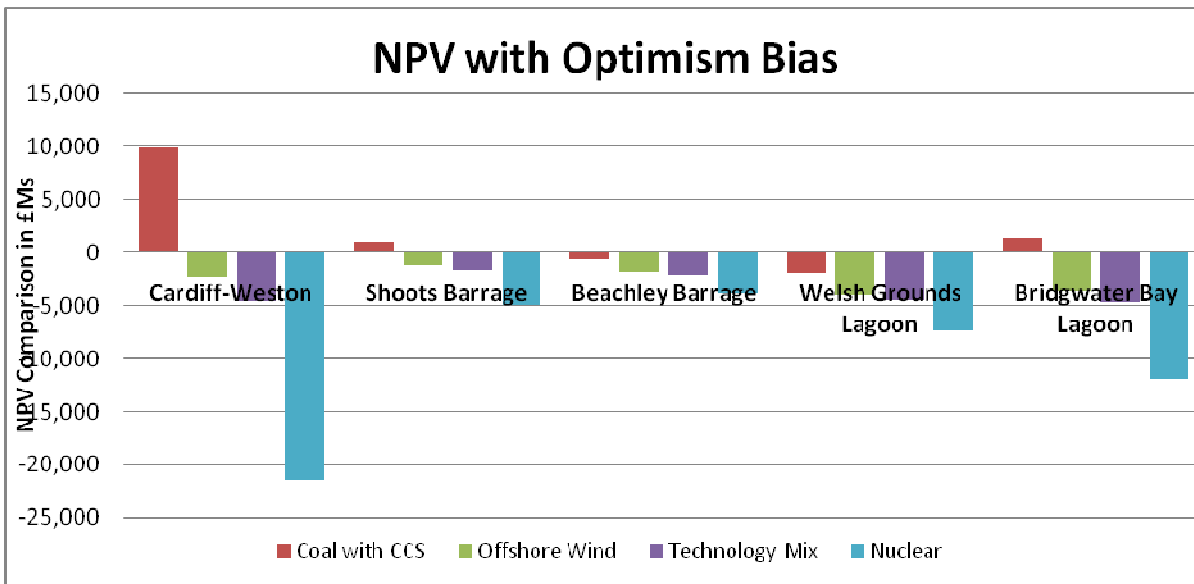
Figure 8: Graph showing the net present value (NPV) of Severn Tidal Power against a range of low carbon technologies.
