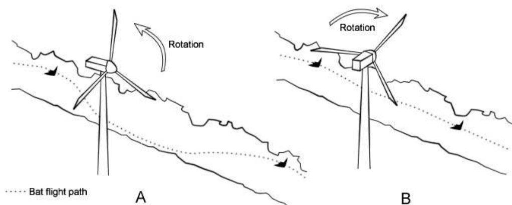
Figure 2.31- Demonstrating how the flight path of the common pipistrelle along a nearby (<10 m) hedgerow changes in accordance with rotor angle; perpendicular (A) and parallel (B). Note that the dip in flight path A when the rotor blades are perpendicular occurs in both directions along the hedgerow (Bach, 2007) (Adapted from Bach & Rahmel, 2004).
