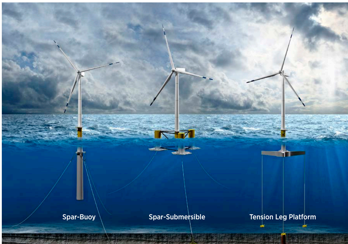
Figure 2-34. Illustrations of three classes of floating wind turbine technology
